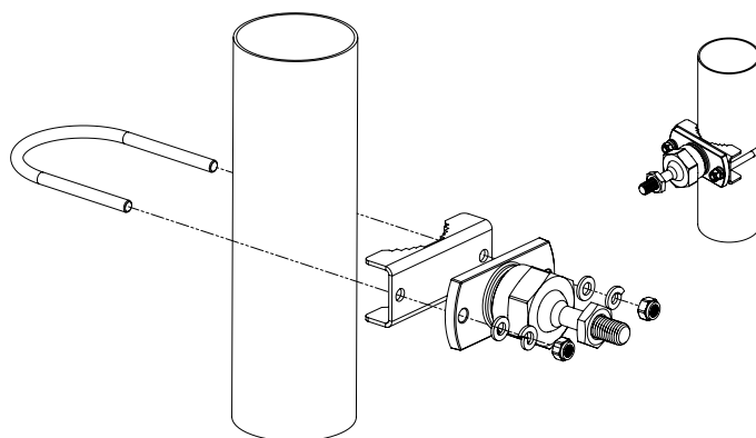
Figure 1 Dimension- and assembly drawing for art. 26803
