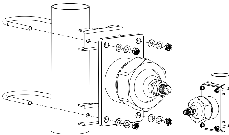
Figure 2 Dimension- and assembly drawing for art. 26807
